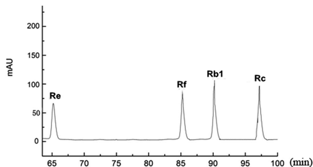
Fig. 2 The retention time of different ginsenosides. (The mixture of standards of individual dammarane. Ginsenosides in the root were analyzed by HPLC and were separated at different time points.)
