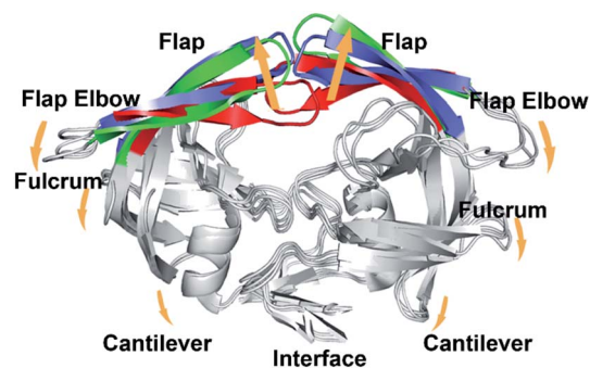
Fig. 1 Superposition of the crystal structures of the closed (3IXO), semi-open (1HHP), and wide-open (1TW7) forms of HIV-1 PR. Arrows indicate the direction of changes during the flap opening.
