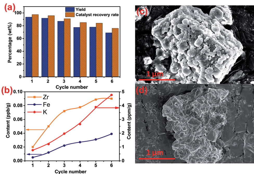
Fig. 11 (a) Reusability of the magnetic catalyst \text{K/ZrO}_2/\gamma\text{-Fe}_2\text{O}_3 (b) accumulation of the Zr, Fe and K elements in the prepared biodiesel (c) SEM result of the initial catalyst \text{K/ZrO}_2/\gamma\text{-Fe}_2\text{O}_3 (d) SEM result of the catalyst \text{K/ZrO}_2/\gamma\text{-Fe}_2\text{O}_3 after six times of use (transesterification conditions: reaction temperature: 65 °C; methanol/oil: 10 : 1; catalyst amount: 5 wt%; reaction time: 3 h).
