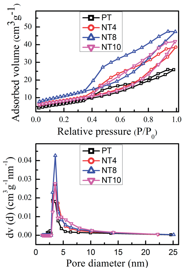
Fig. 2 N 2 adsorption–desorption isotherms (a) and pore diameter distribution curve (b) of PT, NT4, NT8 and NT10 calcined at 450 °C.
