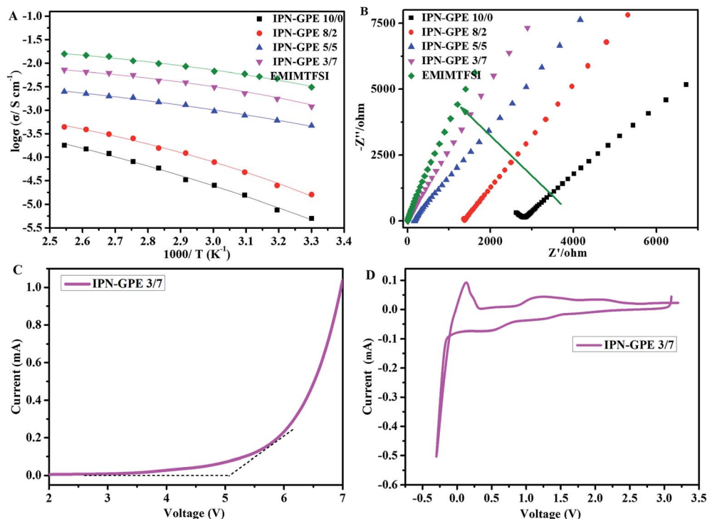
Fig. 4 (A) Temperature dependence of ionic conductivity and (B) impedance spectra of IPN-GPE in various proportion; (C) linear sweep voltammetry curve and (D) cyclic voltammety curve (open circuit potential to -0.3 V) of IPN-GPE 3/7.
