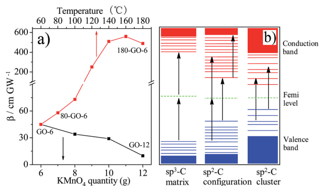
Fig. 9 The nonlinear absorption coefficient \beta of GO- X ( X = 6, 8, 10 and 12 ) and Y-rGO-6 ( Y = 80, 100, 120, 140, 160 and 180 ) as a function of oxidation and reduction degree (a) and representative band structure with related hybrid carbon structure (b).
