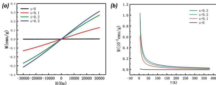
Fig. 7 (a) The magnetic hysteresis loops of the Bi 7 Ti 4-2x Co x Nb 1+x O 21 ( x = 0, 0.1, 0.2, and 0.3 ) ceramics at 10 K. (b) The temperature dependence of magnetization of the samples in the ZFC-FC modes measured at 500 Oe.
