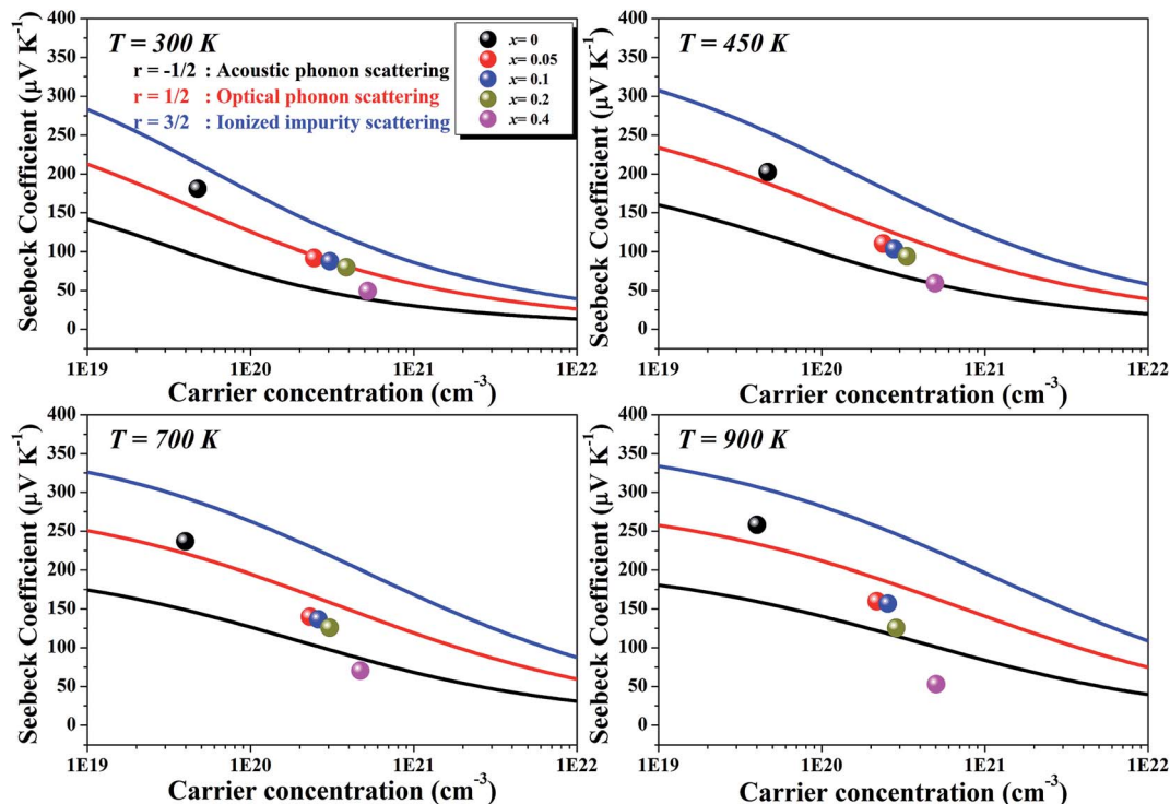
Fig. 6 Calculated carrier concentration-dependent Seebeck coefficients of \text{Li}_{1-x}\text{NbO}_2 ( x = 0, 0.05, 0.1, 0.2 and 0.4 ) samples at various temperatures.
