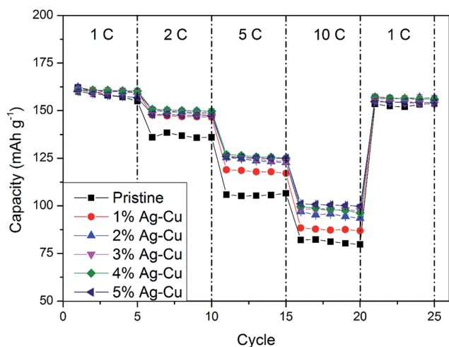
Fig. 9 Rate capability of \text{Li}_4\text{Ti}_5\text{O}_{12}/\text{Ag-Cu} composites.
