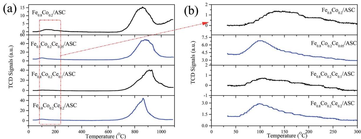
Fig. 5 SO 2 -TPD profiles of catalysts.
