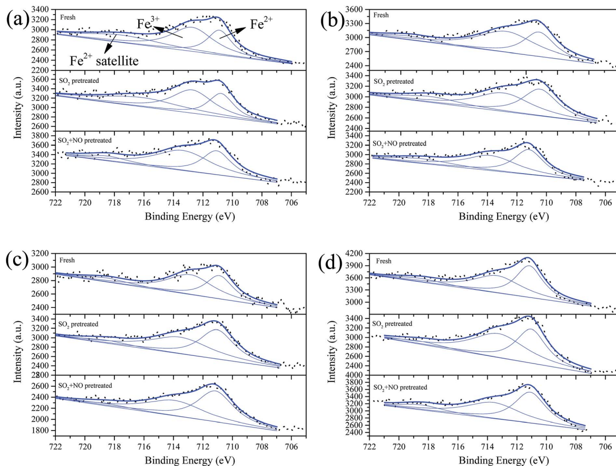
Fig. 6 Fe 2p 3/2 from XPS spectra of catalysts (a) Fe 0.8 Co 0.2 /ASC, (b) Fe 0.8 Co 0.2 Ce 0.05 /ASC, (c) Fe 0.8 Co 0.2 Ce 0.1 /ASC, and (d) Fe 0.8 Co 0.2 Ce 0.2 /ASC, with different treatment.
