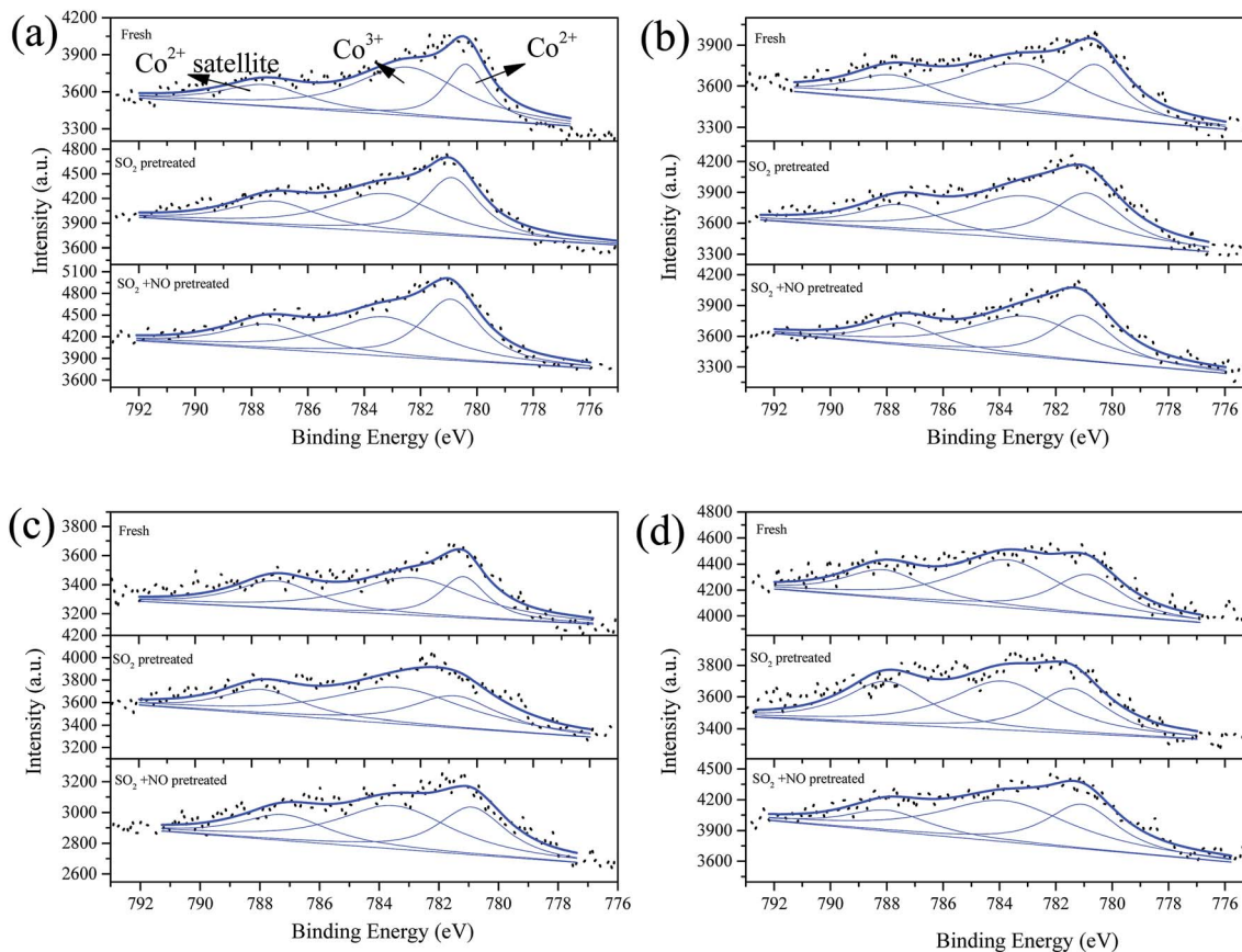
Fig. 7 Co 2p_{3/2} from XPS spectra of catalysts (a) \text{Fe}_{0.8}\text{Co}_{0.2}/\text{ASC} , (b) \text{Fe}_{0.8}\text{Co}_{0.2}\text{Ce}_{0.05}/\text{ASC} , (c) \text{Fe}_{0.8}\text{Co}_{0.2}\text{Ce}_{0.1}/\text{ASC} , and (d) \text{Fe}_{0.8}\text{Co}_{0.2}\text{Ce}_{0.2}/\text{ASC} , with different treatment.
