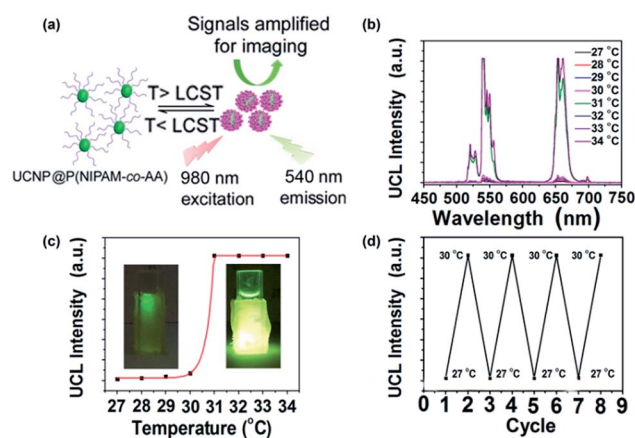
Fig. 2 (a) Illustration of thermoresponsive upconversion emission of UCNP@P(NIPAM-co-AA); (b) UCL spectrum of UCNP@P(NIPAM-co-AA) dispersed in aqueous solution at different temperature under the excitation at 980 nm; (c) UCL intensity as a function of temperature for UCNP@P(NIPAM-co-AA) covered with 2 mm chicken; (d) several cycles of dynamic heating and cooling, showing the repeatability of the upconversion emission intensity with concentration 1 mg mL -1 .
