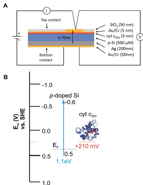
Fig. 6 Construction of the cyt c 553 /Si bioelectrodes. (A) Diagrammatic representation of the all-solid state cyt c 553 /Si bioelectrodes. The thickness (nm or μm) of each layer, measured by sputtering detection, is indicated. The thickness of the Si wafer was 500 μm. (B) Energy band diagram of the cyt c 553 /Si bioelectrode. Indicated are valence (0.5 V vs. NHE) and conduction (−0.6 V vs. NHE) bands for the p-doped Si substrate, and cyt c 553 redox mid potentials ( E_m ) together with the estimated Fermi level ( E_F ) for the used level of boron doping in Si.
