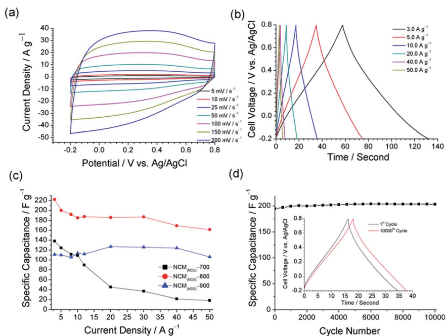
Fig. 8 (a) Cyclic voltammograms of \text{NCM}_{(\text{MDE})-800} in 1.0 M \text{H}_2\text{SO}_4(\text{aq}) at different scan rates from 5 to 200 \text{ mV s}^{-1} . (b) Galvanostatic charge–discharge curves for \text{NCM}_{(\text{MDE})-800} at current density values ranging from 3 to 50 \text{ A g}^{-1} . (c) Specific capacitances of \text{NCM}_{(\text{MDE})-X} at different current densities. (d) Cyclic stability test: specific capacitance calculated from discharge curves of 10 000 cycles at a current density of 10 \text{ A g}^{-1} ; (inset) galvanostatic charge–discharge curves of the 1 st and 10000 th cycles for \text{NCM}_{(\text{MDE})-800} at a current density of 10 \text{ A g}^{-1} .
