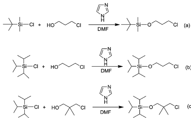
Scheme 3 Synthesis routes of TBDMSOPrCl, TIPSOPrCl and TIPSODMPPrCl.
