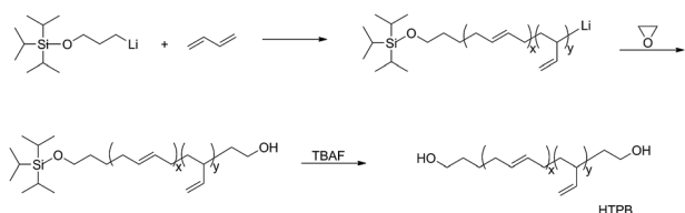
Scheme 7 The synthesis routes of HTPB via anionic polymerization initiated by TIPSOPrLi.
