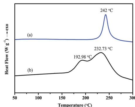
Fig. 4 DSC thermograms of (a) BA-AN and (b) BA-PADPA.
