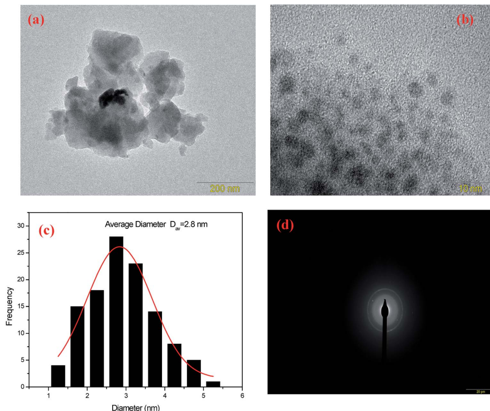
Fig. 4 (a) TEM images (b) at 10 nm scale, (c) particle size distribution curve and (d) selected area electron diffraction pattern (SAED) of Ag5 glass samples.
