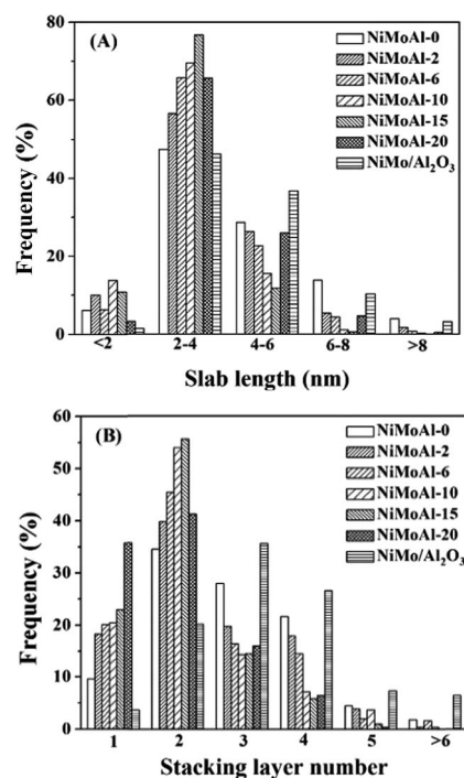
Fig. 4 Slab lengths (A) and stacking layer number (B) distributions of \text{MoS}_2 crystallites on the sulfide \text{NiMoAl-}x and \text{NiMo/Al}_2\text{O}_3 catalysts.
