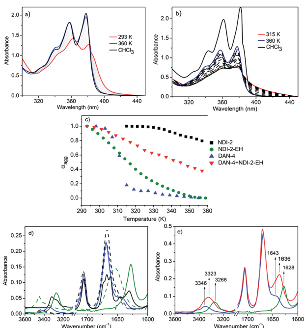
Fig. 2 Variable temperature UV/Vis spectra of (a) NDI-2-EH and (b) NDI-2 in methylcyclohexane ( c = 0.1\text{ mM} ). (c) Melting curves for various self-assembling systems in methylcyclohexane. (d and e) Solvent dependent FT-IR spectra (dotted line- \text{CHCl}_3 , solid line-methylcyclohexane) of NDI-2-EH (blue), NDI-2 (black), DAN-4 (green) and NDI-2-EH + DAN-4 (1 : 1) (red).
