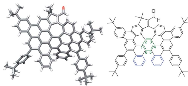
Fig. 3 Distorted graphene molecule 2 : single crystal structure (left) and corresponding ChemDraw structure (right).
