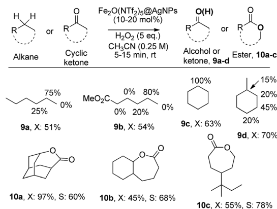
Fig. 6 Redox-catalyzed selective \text{CH}_2 and Baeyer–Villiger oxidations with \text{Fe}_2\text{O}(\text{NTf}_2)_5@AgNPs (10 and 20 mol% of Fe for alkanes and ketones, respectively). X: conversion. S: selectivity. GC results.
