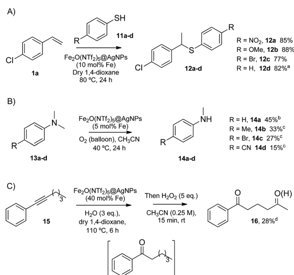
Fig. 7 Acid/redox reactions catalysed by \text{Fe}_2(\text{NTf}_2)_5\text{O}@AgNPs . Isolated yields. From top to bottom: hydrothiolation of styrenes, demethylation of N,N -dimethylanilines, and one-pot hydration of alkyne 15 – \text{CH}_2 oxidation. a After 8 uses of \text{Fe}_2(\text{NTf}_2)_5\text{O}@AgNPs . b Combined yield with the corresponding trimers. c Combined yield with the corresponding formamides. d GC yield.
