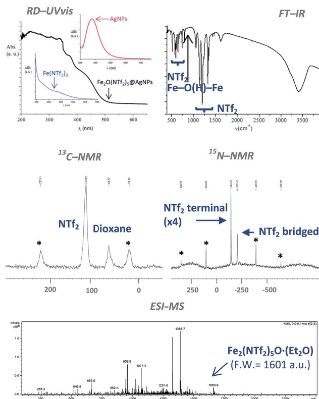
Fig. 3 Top: Fourier transform-infrared (FT-IR) and diffuse reflectance ultraviolet-visible (RD-UV vis) spectra of the \text{Fe}_2\text{O}(\text{Ntf}_2)_5\text{@AgNPs} solid. For the sake of comparison, the UV-vis spectra of \text{Fe}(\text{Ntf}_2)_3 and 10 nm Ag nanoparticles in solution are also shown. Middle: ^{13}\text{C} and ^{15}\text{N} nuclear magnetic resonance-magic angle spinning (NMR-MAS) spectra of the ^{15}\text{N} isotopically-labelled yellow solid (* = rotational peaks). Bottom: electrospray ionization mass spectrum (ESI-MS) of the solid extracted with diethyl ether.
