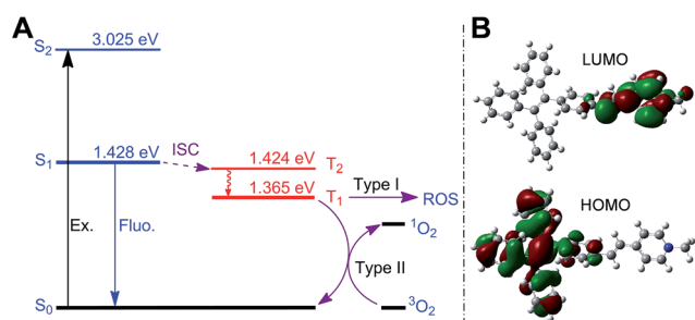
Fig. 3 (A) Energy diagrams of TPE-Py-Me as calculated using TD-DFT and the proposed pathway of ROS generation. The energy level of ground state was set to zero. (B) Electron density distribution of the HOMO and LUMO of TPE-Py-Me based on the geometry of the excited state calculated using the B3LYP/6-31G* basis set. TPE-Py-Me is adopted as a representative of TPE-Py in the calculation model for simplicity.
