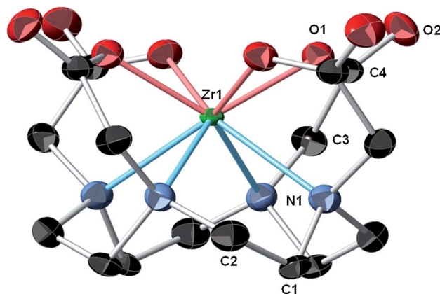
Fig. 2 Crystal structure of \text{Zr} -DOTA.† Thermal ellipsoids are drawn at the 50% probability level; only one of the crystallographically-independent \text{Zr} centers is shown and a partial atomic labeling scheme is provided. The disordered \text{Zr} center, disordered solvent molecules, and hydrogen atoms are omitted for clarity.
