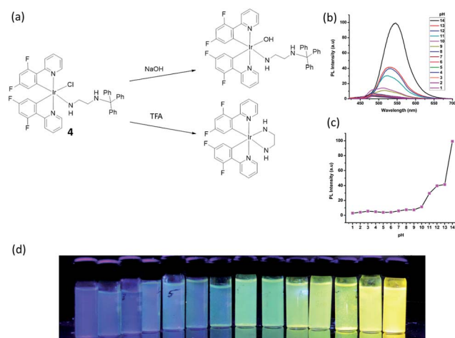
Fig. 4 (a) Chemical structure of 4 and reactions with NaOH or TFA. (b) The pH-Dependent luminescent spectra of 4 with different pH buffer solution (THF/buffer, 1 : 9). (c) The pH-Dependent intensity plot at different pH values. (d) Fluorescent photos of 4 at different pH values at 365 nm. 53 Reprinted figures with permission from Copyright (2015) American Chemical Society.
