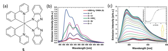
Fig. 5 (a) Chemical structure of complex 5 . (b) Luminescence intensity of IrBBI- \text{H}_2 \cdots \text{DNBA} with 110 equiv. of different anions. (c) Luminescence of IrBBI- \text{H}_2 \cdots \text{DNBA} as a function of different concentration of fluoride; inset: plot of the normalized IrBBI- \text{H}_2 \cdots \text{DNBA} luminescence response as a function of the number of equivalents of fluoride added. 54 Reprinted figures with permission from Copyright (2015) Royal Society of Chemistry.
