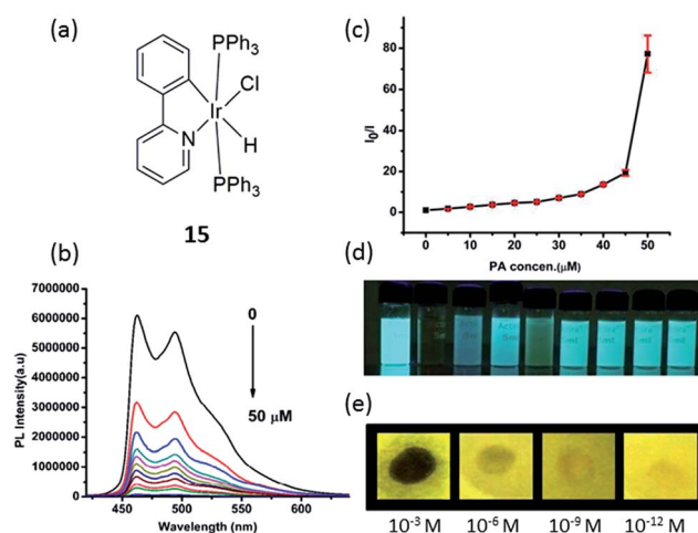
Fig. 15 (a) Chemical structure of complex 15 . (b) Photoluminescence spectra of 15 in THF–water ( v/v = 1 : 9 ) with different amounts of PA. (c) Corresponding Stern–Volmer plots of PA. (d) Image of 15 ( 10 \mu\text{M} ) when dispersed in THF–water ( v/v = 1 : 9 ) with addition of 5 equivalents of each explosive/non explosive compounds, respectively (from left to right: blank, PA, 3,5-dinitrotoluene, nitrobenzene, 2,4-DNP, 1,3-dinitrobenzene, nitrobenzene, toluene and benzoic acid). (e) Luminescent photographs of paper plates impregnated by 15 against different concentrations of PA. 84 Reprinted figures with permission from Copyright (2015) Royal Society of Chemistry.
