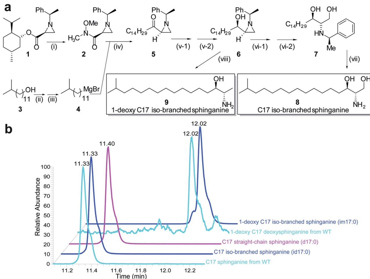
Fig. 2 C17 iso-branched sphingoid bases as analytical standards. (a) Synthetic route for nematode C17 iso-branched sphinganine (8) and its 1-deoxy analogue (9): (i) Weinreb's amine, AlMe 3 , CH 2 Cl 2 , –10 °C, 30 min, then rt, 2 h, 45%; (ii) PPh 3 /Br 2 , pyridine/CH 2 Cl 2 , 3 h, rt, 88%; (iii) Mg, I 2 , dry THF, 20 min, 66 °C, quantitative yield; (iv) THF, –78 °C, 30 min, 45%; (v-1) ZnCl 2 , MeOH, –78 °C, 30 min; (v-2) NaBH 4 , 30 min, –78 °C, 80%; (vi-1) AcOH, CH 2 Cl 2 , rt, 18 h; (vi-2) KOH, EtOH, rt, 1.5 h; (vii) H 2 , Pd/C, MeOH, rt, overnight, 58%; (viii) H 2 , Pd(OH) 2 /C, MeOH, rt, overnight, 42%; (b) LC-MS profiles of endogenous C17 sphinganine and 1-deoxy C17 sphinganine from WT C. elegans , synthesized iso-branched C17 bases, and commercial C17 straight-chain sphinganine. Retention times are indicated above each peak.
