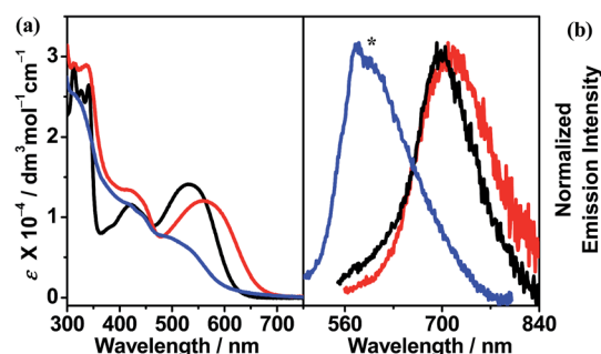
Fig. 3 (a) UV-vis absorption and (b) emission spectra ( [\text{Pt}] \approx 1 \times 10^{-5} \text{ M} ) of (—) 1 , (—) 2 and (—) mononuclear complex in \text{CH}_2\text{Cl}_2 at 298 K. (The asterisk indicates the instrumental artifact.)
