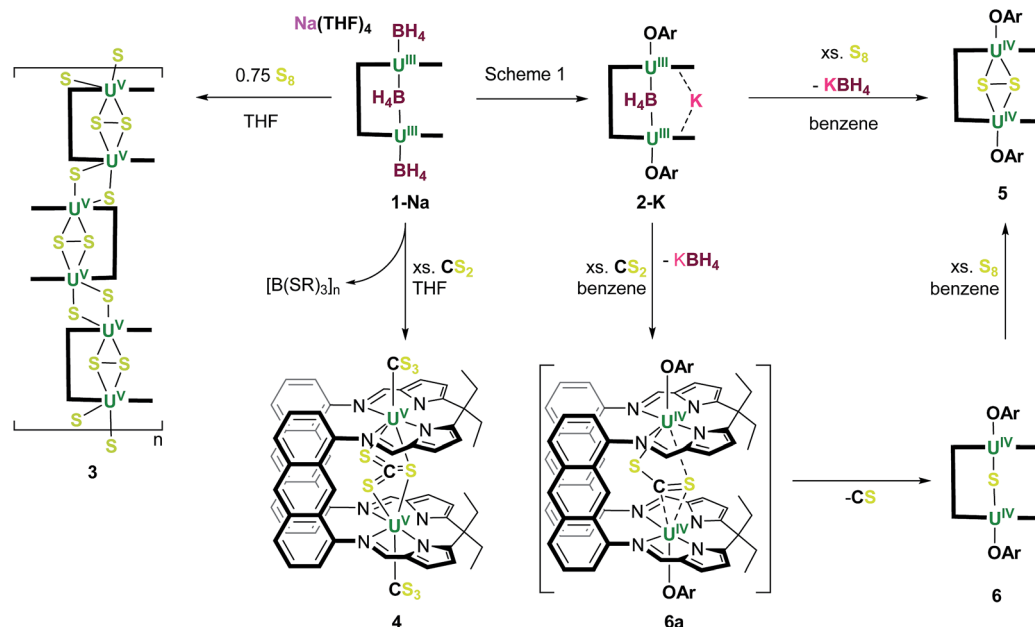
Scheme 2 Contrasting reactions of [\text{Na}(\text{THF})_4][\{\text{U}(\text{BH}_4)_2(\mu\text{-BH}_4)(\text{L}^{\text{A}})(\text{THF})_2\}] ( 1-Na ) and [\{\text{U}(\text{OAr})(\text{THF})_2\}_2(\text{endo-}\mu\text{-KBH}_4)(\text{L}^{\text{A}})] ( 2-K ) and the synthesis of complexes 3–6 (OAr = \text{OC}_6\text{H}_2^t\text{Bu}_{3-2,4,6} ).
