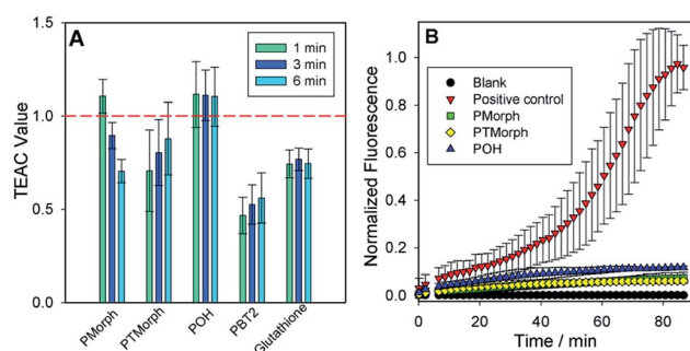
Fig. 3 (A) Trolox-Equivalent Anti-oxidant Capacity (TEAC) values at 1, 3, and 6 minutes for Trolox, PBT2, glutathione, and each phenol-triazole ligand. Each experiment was completed in triplicate and error bars represent \pm\text{SD} for the average TEAC values. Note: PBT2 shows weak anti-oxidant capacity in TEAC assay most likely due to electron-withdrawing chloride substituents in the ortho/para positions. (B) A fluorogenic assay monitoring the production of 7-hydroxyCCA over time. In the absence of any exogenous ligands, free Cu exhibits Fenton-like chemistry to produce hydroxyl radicals, which react with CCA to form a fluorescent product. Introduction of POH, PMorph, or PTMorph to a solution containing CCA, Cu, and ascorbate, a distinct inhibition in fluorescent product is observed. Conditions: 40 \mu\text{M} \text{CuSO}_4 , 100 \mu\text{M} CCA, 80 \mu\text{M} ligands, 400 \mu\text{M} L-ascorbic acid, \lambda_{\text{ex}} : 395 nm/ \lambda_{\text{em}} : 450 nm.
