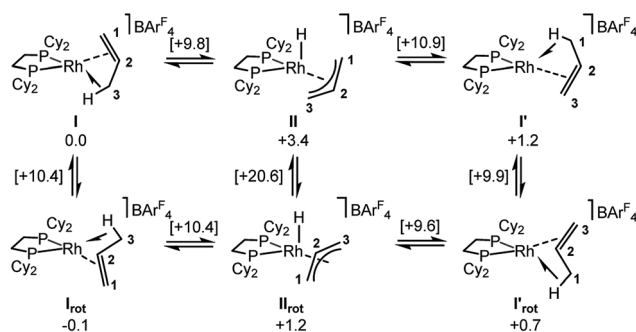
Scheme 10 Computed mechanisms for fluxionality and D-label scrambling in [\mathbf{1}\text{-}(\text{propene})][\text{BAR}^F_4] in the solid-state. Gibbs free energies are indicated in kcal \text{mol}^{-1} with those for transition states provided in square brackets.
