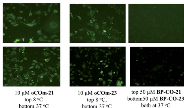
Fig. 4 CO specific fluorescent probe (COP-1) confirms increased intracellular CO levels following exposure to oCOM-21 (10 \mu M) or oCOM-23 (10 \mu M) against the respective iCORM (50 \mu M) at both 37 ^{\circ} C and 8 ^{\circ} C.
