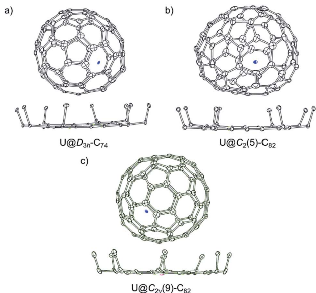
Fig. 2 ORTEP drawings showing the relative orientations of the uranium endohedrals and porphyrin for (a) \text{U@D}_{3h}\text{-C}_{74} \cdot \text{Ni}^{\text{II}}(\text{OEP}) \cdot 2(\text{toluene}) , (b) \text{U@C}_2(5)\text{-C}_{82} \cdot \text{Ni}^{\text{II}}(\text{OEP}) \cdot 2(\text{toluene}) and (c) \text{U@C}_{2v}(9)\text{-C}_{82} \cdot \text{Ni}^{\text{II}}(\text{OEP}) \cdot 1.5(\text{toluene}) \cdot \text{CS}_2 . Thermal ellipsoids are shown at the 10% probability level. Only the major fullerene cage and the predominant uranium orientation are shown, and minor sites and solvent molecules are omitted for clarity.
