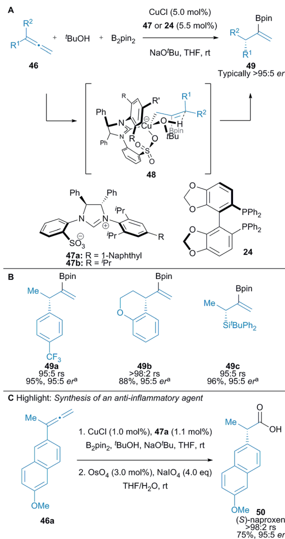
Scheme 8 Hoveyda's borocupration of allenes and subsequent protonation of the allyl copper intermediate. rs = regioselectivity ( \gamma/\alpha site selectivity of protonation). a using 47a .
