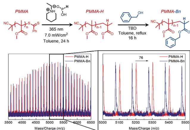
Fig. 4 Matrix assisted laser desorption/ionization time-of-flight mass spectrometry (MALDI-TOF-MS) spectrum of chain-end selective transesterification of end-group removed PMMA (PMMA-H, red) resulting in terminal functionalized PPMA (PMMA-Bn, blue).
