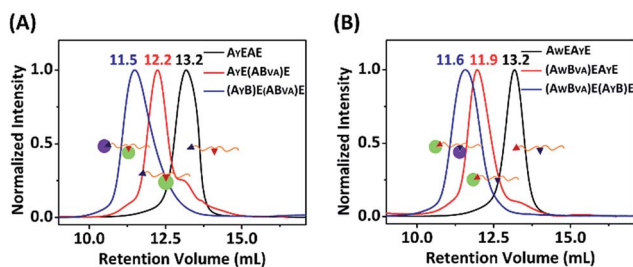
Fig. 6 SEC overlay of the products at each stage from the sequential reaction of A Y EA E (left) or A W EA Y E (right), firstly with B VA and then with B. The numbers above the peaks denote the retention volume of each peak.
