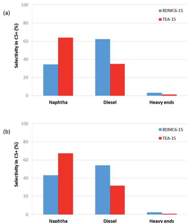
Fig. 14 Selectivity within the accumulated C_5^+ liquid fractions for the nanosized beta catalysts at WHSV = 14.3 \text{ h}^{-1} , T = 200 \text{ }^\circ\text{C} , P = 4.0 \text{ MPa} , 60% mol olefin in the feed. (a) TOS = 0–3 h, (b) TOS = 3–6 h.
