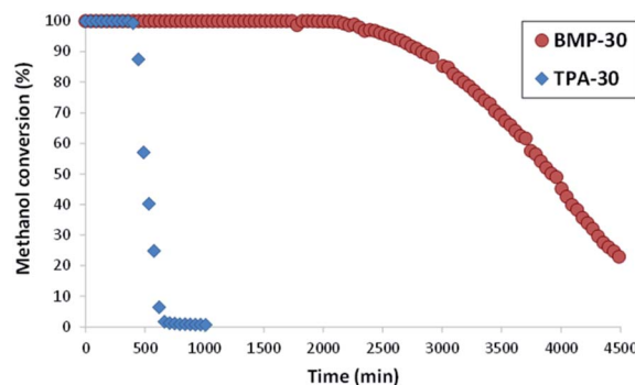
Fig. 8 Conversion of methanol using ZSM-5 catalysts (reaction conditions: T = 450 °C, \text{WHSV} = 10 \text{ h}^{-1} , W_{\text{cat}} = 50 mg).
