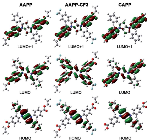
Fig. 6 The Frontier molecular orbitals of AAPP, AAPP-CF 3 and CAPP obtained via DFT calculations. The geometries were optimized with the M06-2X density functional and the 6-31G(d,p) basis set. The value of the contour envelopes is 0.03 au.
