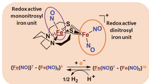
Fig. 1 Structure and redox activity of [(\text{NO})\text{FeN}_2\text{S}_2\cdot\text{Fe}(\text{NO})_2]^+ , [\text{Fe}-\text{Fe}]^+ ; protonation of the one-electron reduced diiron complex yields \text{H}_2 . 8
