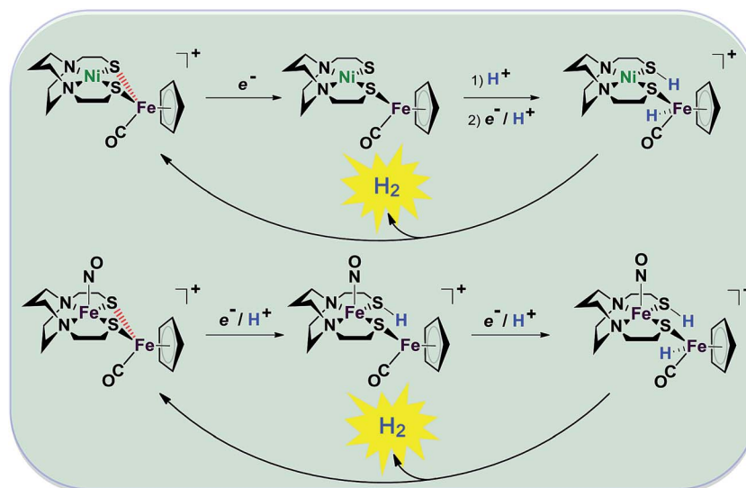
Fig. 2 Abbreviated computational mechanisms for electrocatalysis of \text{H}_2 production by the [\text{Fe}-\text{Fe}]^+ and [\text{Ni}-\text{Fe}]^+ electrocatalysts. 9 Shown in red is the \text{Fe}-\text{S} bond that undergoes reductive bond cleavage.
