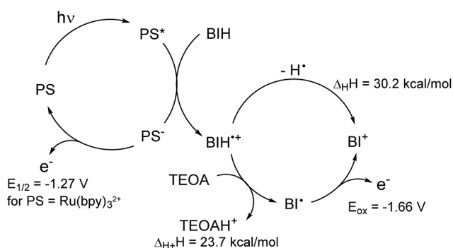
Scheme 3 Proposed photoexcitation scheme involving a BIH sacrificial donor. Enthalpy changes in hydrogen atom and proton transfer, as well as E_{ox} (BI • ), were determined in ref. 44, E_{1/2} (Ru(bpy) 3 2+/•+ ) value is given in ref. 45. Redox potentials are given vs. SCE.
