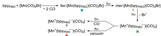
Scheme 2 Proposed photolysis pathway of [Mn(bpy_{PMO})(CO)_3Br] species.
