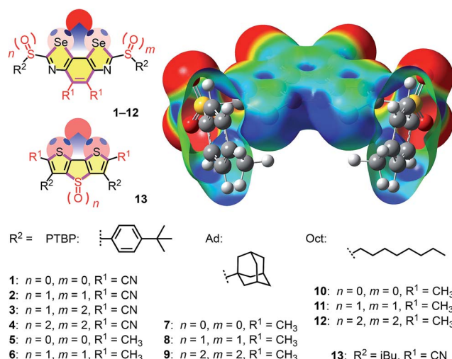
Fig. 1 The BDS (top, 1–12) and DTT motif (bottom, 13) with electron-rich chalcogen-bond acceptors (red) bound in the focal point of the \sigma holes (blue), together with the semitransparent cutaway molecular electrostatic potential (MEP) surface of 4' ( R^2 = \text{pMePh} , MP2/6-311++G**//M062X/6-311G**, isosurface: 0.008 au; red: -0.010 \text{ au} , blue: 0.096 \text{ au} ). 22
