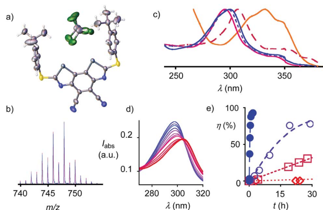
Fig. 3 (a) Crystal structure of 1 with \text{CHCl}_3 . (b) Simulated (pink) and measured ESI mass spectrum of 4 (blue). (c) Normalized absorption spectra of 2 , 3 , 4 , 1 and 5 in THF (increasing \lambda_{\text{max}} ). (d) Absorption spectra of 2 in THF with increasing concentrations of TBACl (0 to 1.95 mM, blue to red). (e) Conversion \eta of 23a with 30 mol% 1 ( \diamond ), 2 ( \square ), 3 ( \circ ) and 4 ( \bullet ) as a function of time, with trend lines.
