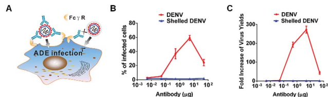
Fig. 4 A CaP nanoshell abrogates the ADE of infection in vitro . (A) Schematic illustration showing that CaP camouflages inhibits antibody recognition and ablates the Fc \gamma R dependent virus infection. (B) DENV or shelled DENV that was first opsonized with serial dilutions of 4G2 was then incubated with K562 cells. The number of DENV-infected cells was measured through flow cytometry. (C) Antibody-enhanced viral production was examined by plaque formation assay. The results were presented as the fold-increase of virus titer after being opsonized with the pre-existing 4G2 antibody.
