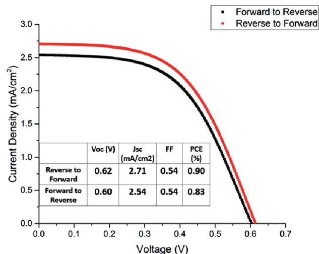
Fig. 10 Boltzmann-fitted J - V curves of the [py][BiI 4 ] champion cell.
