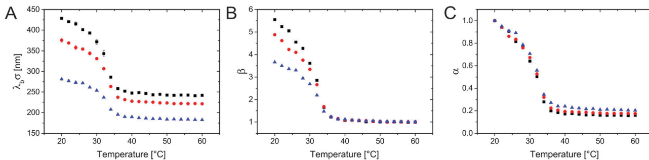
Fig. 2 Results from temperature-dependent DLS measurements for the different core-shell particles: CS 3.4 (black), CS 3.0 (red) and CS 2.2 (blue). (A) Hydrodynamic diameter \lambda_b \sigma as a function of temperature. The error bars are mostly within the symbol size. (B) Temperature-dependent evolution of the swelling ratio \beta = V_{cs}(T)/V_{cs}(60\text{ °C}) . (C) De-swelling ratio \alpha of the hydrogel shells only versus temperature, with \alpha = V_s(T)/V_s(20\text{ °C}) .
