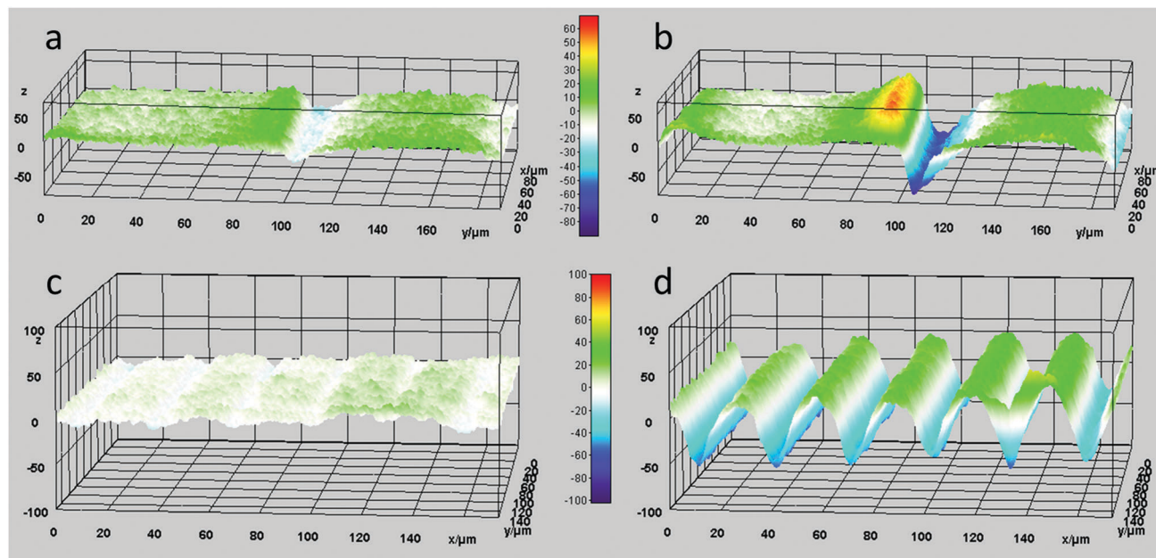
Fig. 5 Snapshots of the videos depicting the 3D image of the coatings captured using digital holographic microscopy. Initial quasi-flat (a and c) and maximum topographic states (b and d) of the coatings with orthogonal 0^\circ/90^\circ patterned domain sizes of 100\ \mu\text{m} (a and b) and 20\ \mu\text{m} (c and d). In snapshot (a and b), the domains oriented 90^\circ are located on the left and 0^\circ on the right of the topological defect line (topography). In snapshot c and d, the domains oriented 0^\circ and 90^\circ are located in the valleys and hills of the coatings, respectively. The viewing position in (a and b) is rotated for a better illustration of the topological defect line.
