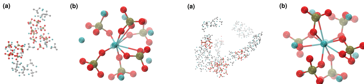
Fig. 8 Solution II: (a) aggregates after 5 ns; (b) detail of one of the Posner-like clusters formed with formula \text{Ca}_9(\text{PO}_4)_6 . Colour key Ca: light blue, P: green, O: red, atoms not forming Posner's clusters: grey.
