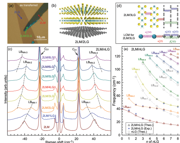
Fig. 30 (a) Optical image of 2LM/2LG vdWHs formed by transferring a 2LM flake on a 2LG flake. (b) Schematic illustration of 2LM/2LG vdWHs. (c) Stokes/anti-Stokes Raman spectra in the region of C and LB modes of pristine 2LM and 2LM/ n LG vdWHs annealed for 30 min. The black dashed lines are eye guides. (d) Schematic diagram of an LCM for the LB modes in 2LM/3LG, in which the next nearest LB coupling in the 3LG constituents is considered. (e) Pos(LB) of n LG and 2LM/ n LG as a function of n of n LG based on the LCM model. The crosses show the experimental Pos(LB) in 2LM/ n LG. Reproduced with permission from ref. 36. Copyright 2017, American Chemical Society.
