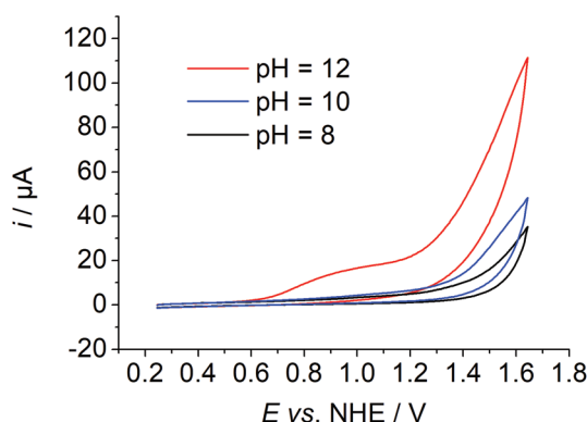
Fig. 2 pH dependent CV data of 1 in Millipore water ( [\mathbf{1}] \approx 1 mM, \nu = 0.1 \text{ mV s}^{-1} , 0.1 \text{ M PO}_4^{3-} , \nu = 0.1 \text{ mV s}^{-1} ).
