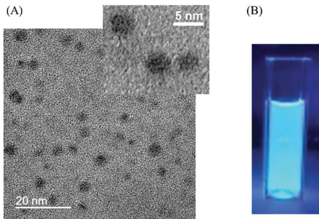
Fig. 1 (A) TEM image of the CDs; (B) photograph of CDs in ethanol with 365 nm excitation.
