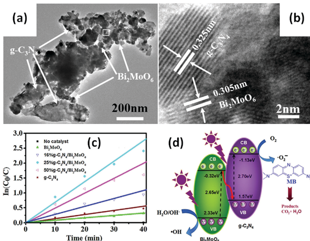
Fig. 30 (a) TEM and (b) HRTEM images of a g\text{-C}_3\text{N}_4/\text{Bi}_2\text{MoO}_6 composite; (c) pseudo first-order fitted kinetic curves of MB degradation on g\text{-C}_3\text{N}_4/\text{Bi}_2\text{MoO}_6 composites (25% g\text{-C}_3\text{N}_4/\text{Bi}_2\text{MoO}_6 ); and (d) a schematic illustration of electron and hole migration in a g\text{-C}_3\text{N}_4/\text{Bi}_2\text{MoO}_6 direct Z-scheme heterojunction. Reproduced with permission from ref. 297. Copyright 2015 Elsevier.
