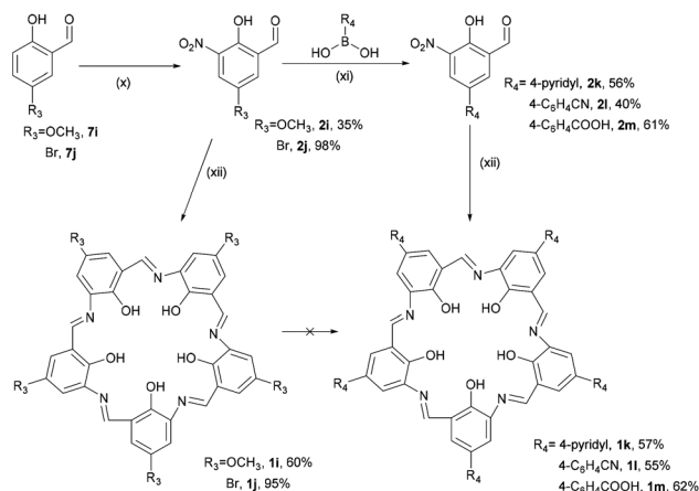
Scheme 2 Syntheses of campestarenes ( 1i–1m ): (x) \text{HNO}_3 , \text{AcOH} , 2 h; (xi) \text{Na}_2\text{CO}_3 , \text{Pd}(\text{PPh}_3)_4 , \text{DMF}/\text{H}_2\text{O} , 105\text{ }^\circ\text{C} , 6 h, then \text{HCl} ; (xii) \text{Na}_2\text{S}_2\text{O}_4 , \text{EtOH}/\text{H}_2\text{O} , reflux, 2 h.
