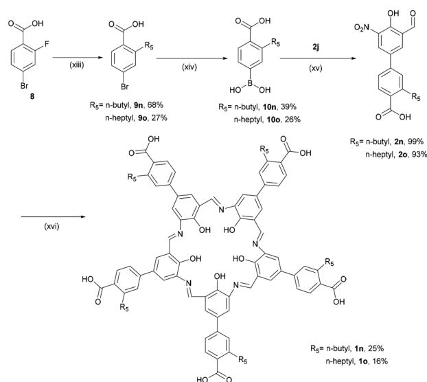
Scheme 3 Syntheses of campestarenes ( 1n and 1o ): (xiii) \text{R}_5\text{MgBr} , \text{THF} , \text{N}_2 , 17 h, then \text{HCl} ; (xiv) n -BuLi, \text{B}(\text{O}-i\text{-Pr})_3 , \text{THF} , -78\text{ }^\circ\text{C} , 3 h, then \text{HCl} ; (xv) \text{Na}_2\text{CO}_3 , \text{Pd}(\text{PPh}_3)_4 , \text{DMF}/\text{H}_2\text{O} , 105\text{ }^\circ\text{C} , 6 h; (xvi) \text{Na}_2\text{S}_2\text{O}_4 , \text{EtOH}/\text{H}_2\text{O} , reflux, 2 h.
