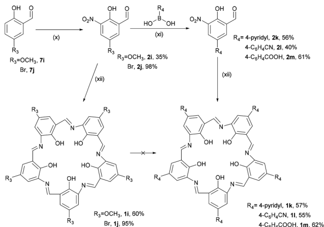
Scheme 2 Syntheses of campestarenes ( 1i–1m ): (x) \text{HNO}_3 , AcOH, 2 h; (xi) \text{Na}_2\text{CO}_3 , \text{Pd}(\text{PPh}_3)_4 , DMF/ \text{H}_2\text{O} , 105 °C, 6 h, then HCl; (xii) \text{Na}_2\text{S}_2\text{O}_4 , EtOH/ \text{H}_2\text{O} , reflux, 2 h.
