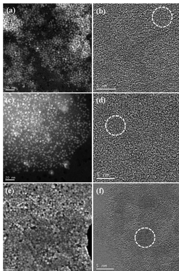
Fig. 1 STEM and HRTEM micrographs for (a and b) ZnO- una 1 NCs (DMSO), (c and d) ZnO- hex 2 NCs (DMSO), and (e and f) ZnO- hex 2 NCs (after 3 days in H 2 O).
